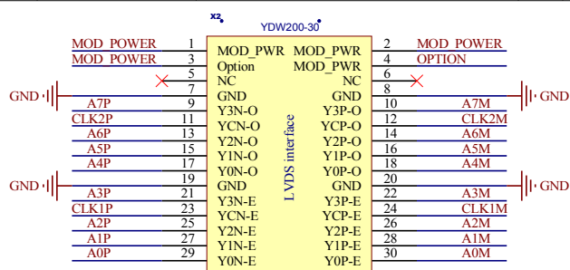
LVDS 30PIN
